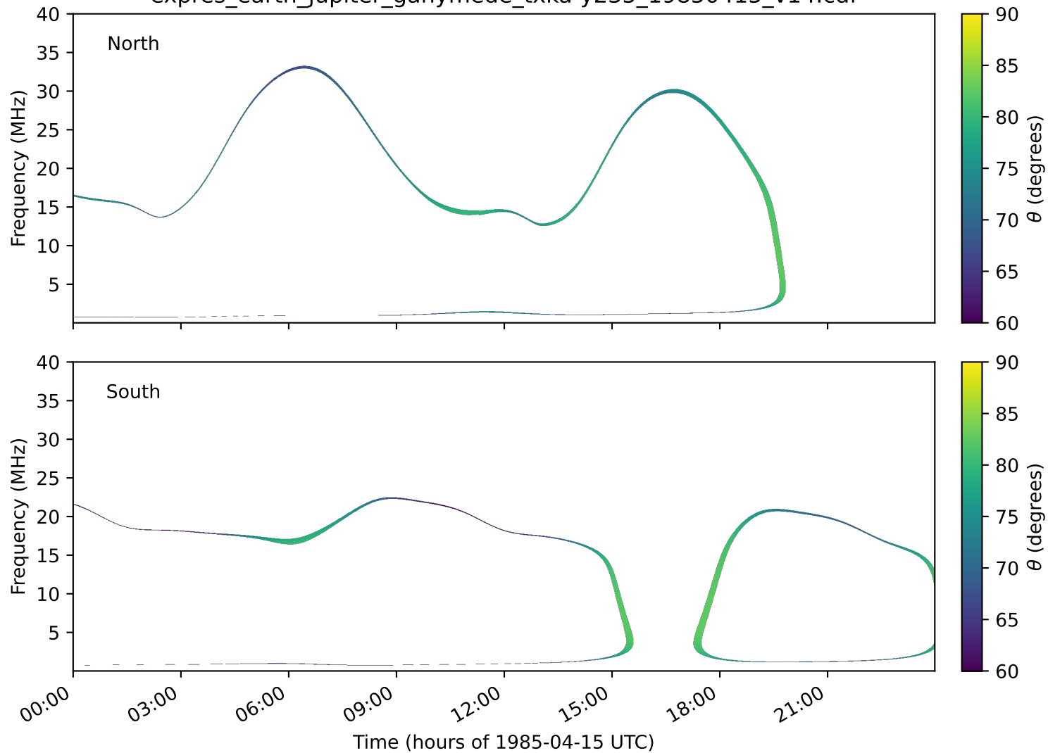
expres_earth_jupiter_ganymede_txka-y235_19850415_v14.cdf
