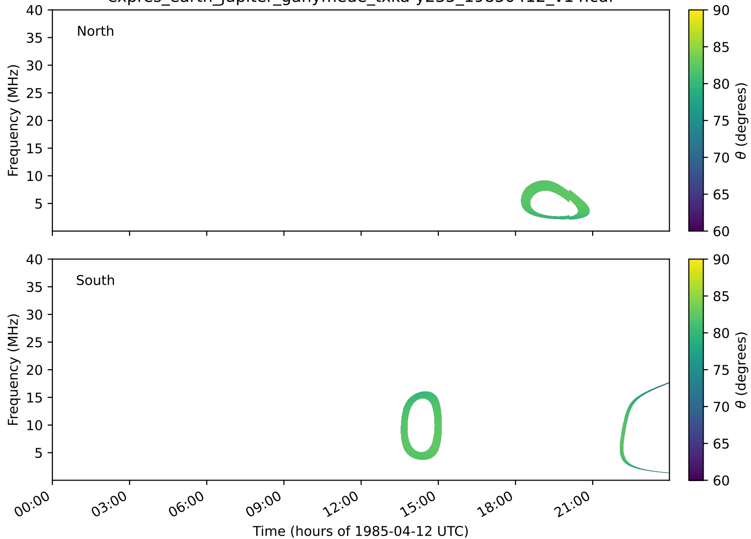
expres_earth_jupiter_ganymede_txka-y235_19850412_v14.cdf
