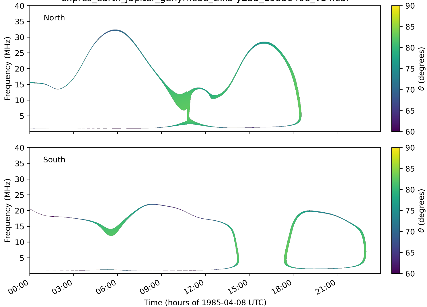
expres_earth_jupiter_ganymede_txka-y235_19850408_v14.cdf
