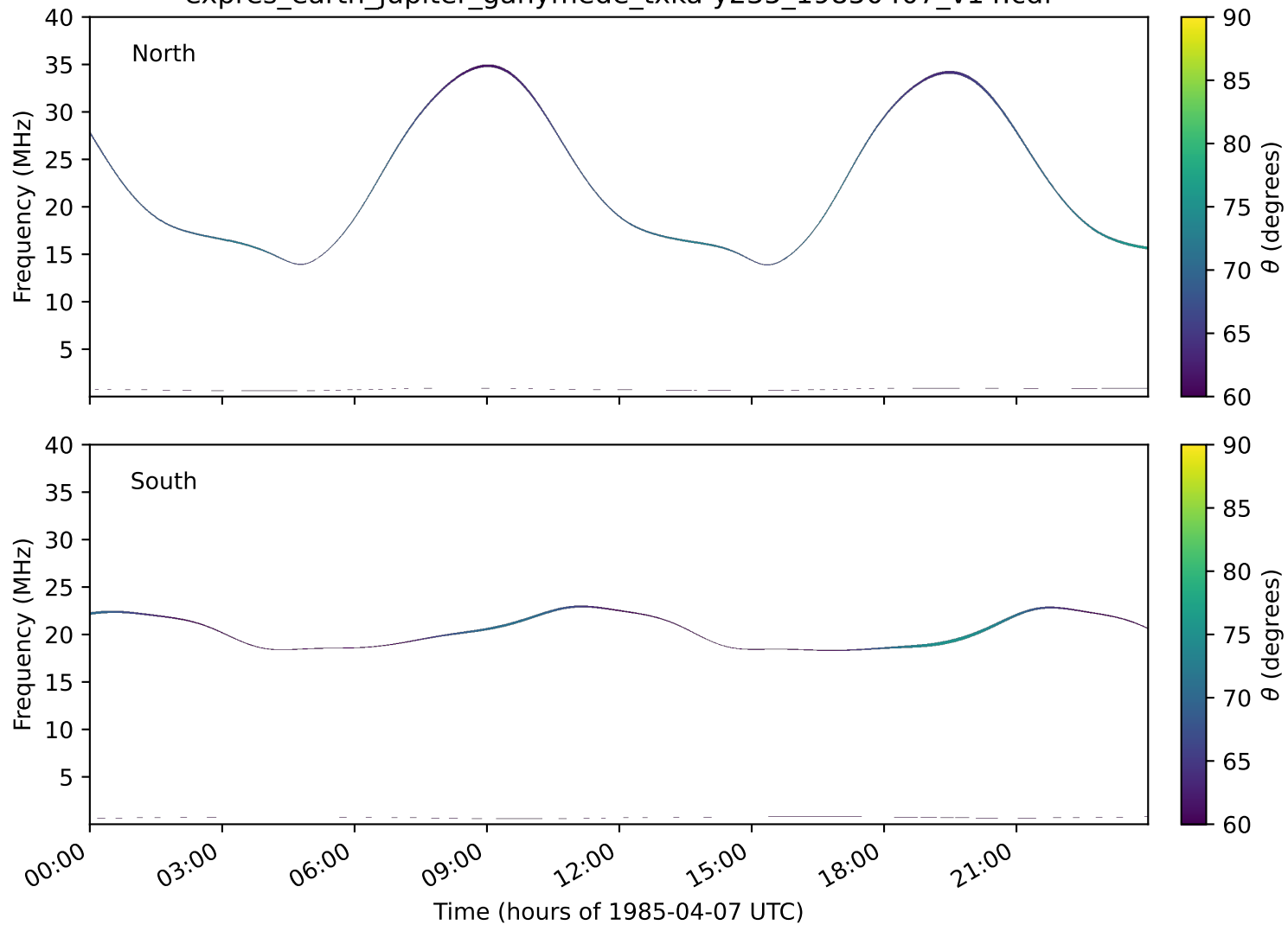
expres_earth_jupiter_ganymede_txka-y235_19850407_v14.cdf
