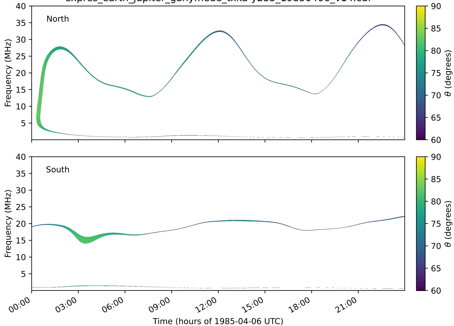
expres_earth_jupiter_ganymede_txka-y235_19850406_v14.cdf
