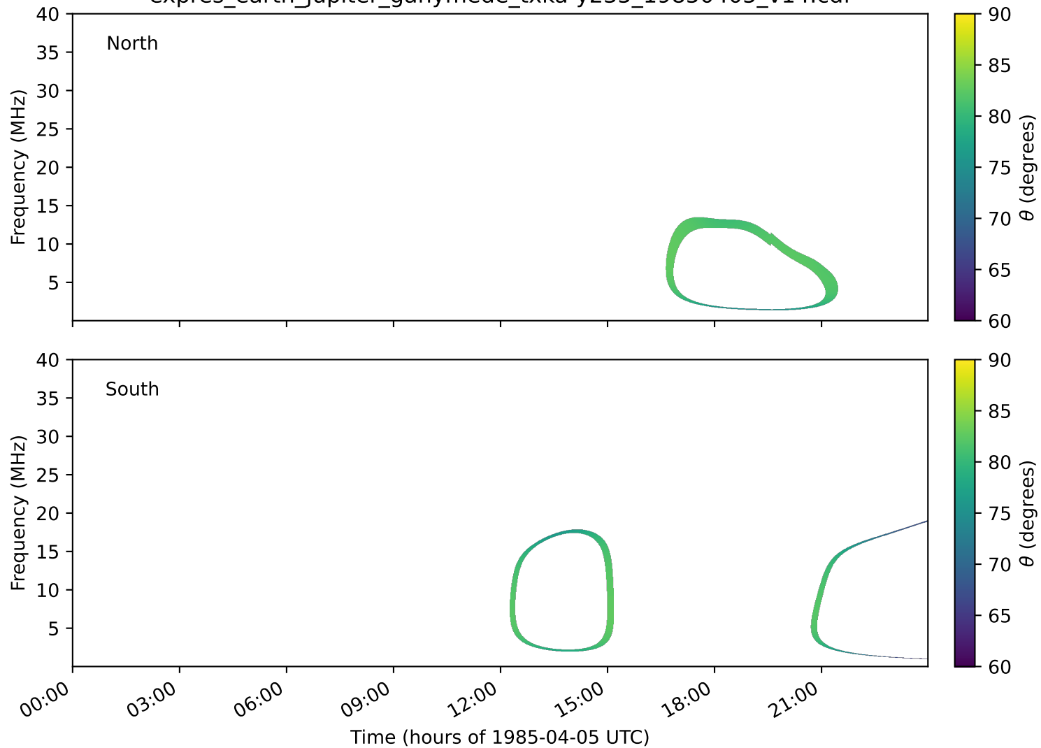
expres_earth_jupiter_ganymede_txka-y235_19850405_v14.cdf
