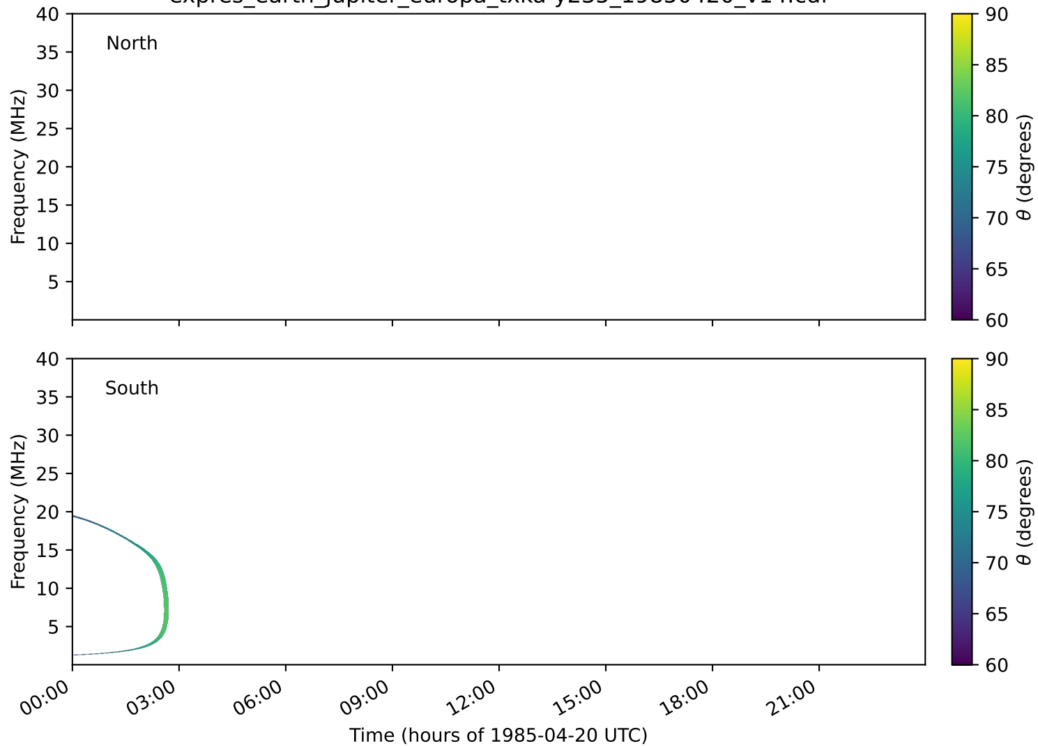
expres_earth_jupiter_europa_txka-y235_19850420_v14.cdf
