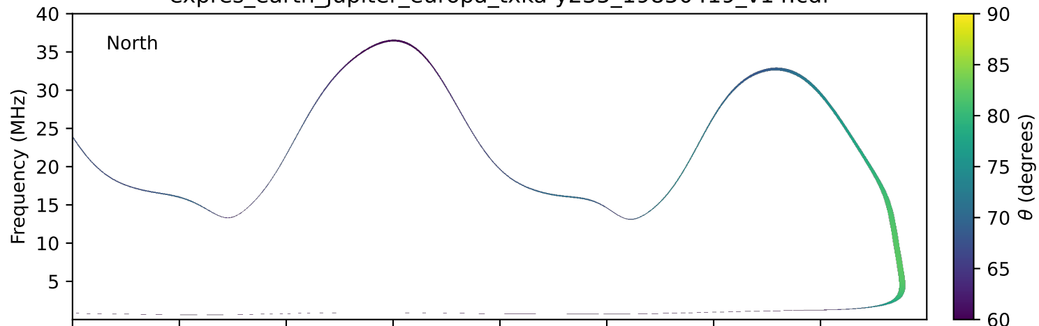
expres_earth_jupiter_europa_txka-y235_19850419_v14.cdf
