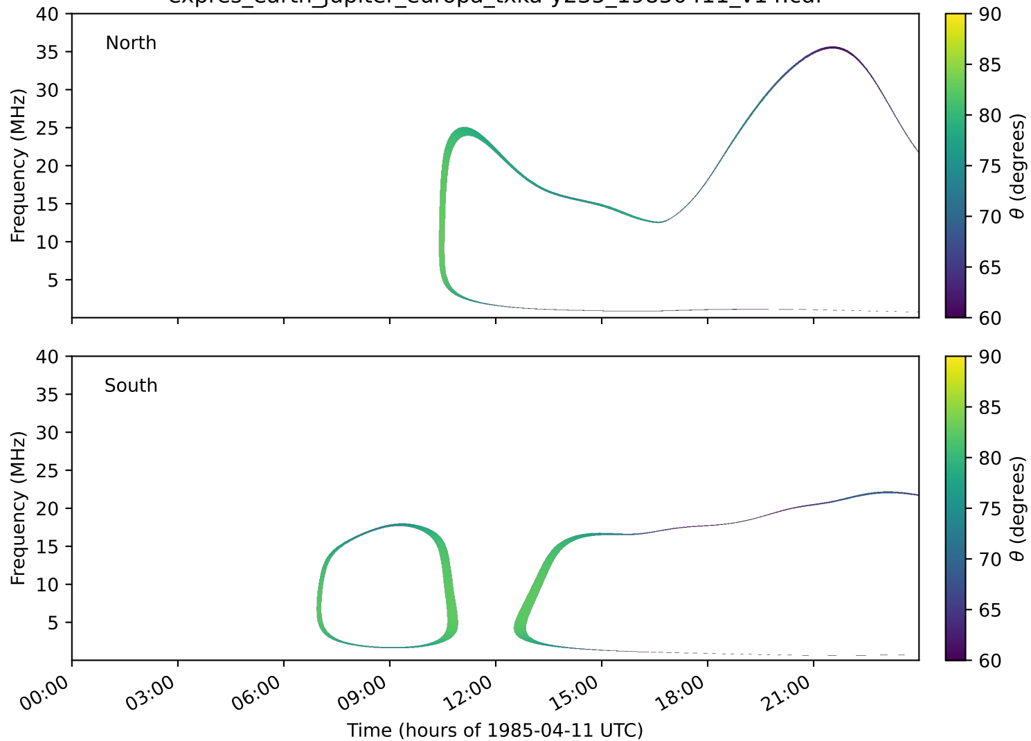
expres_earth_jupiter_europa_txka-y235_19850411_v14.cdf
