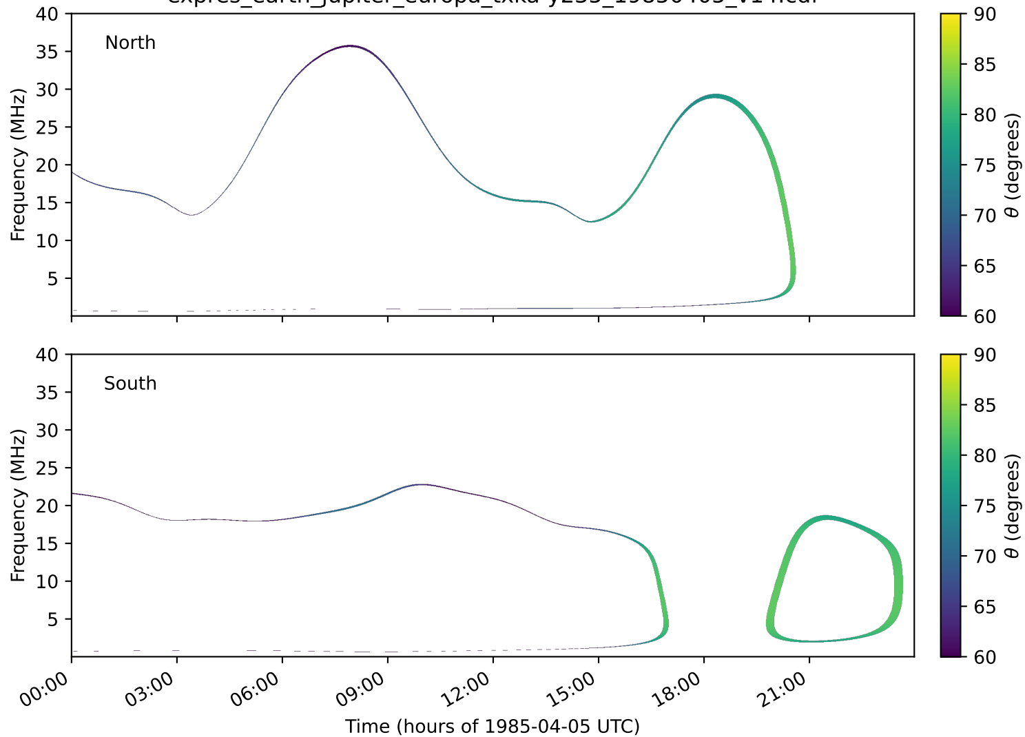
expres_earth_jupiter_europa_txka-y235_19850405_v14.cdf
