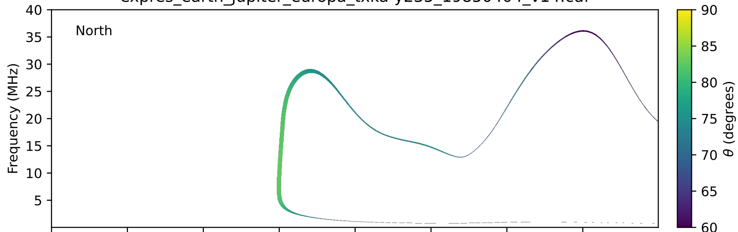
expres_earth_jupiter_europa_txka-y235_19850404_v14.cdf
