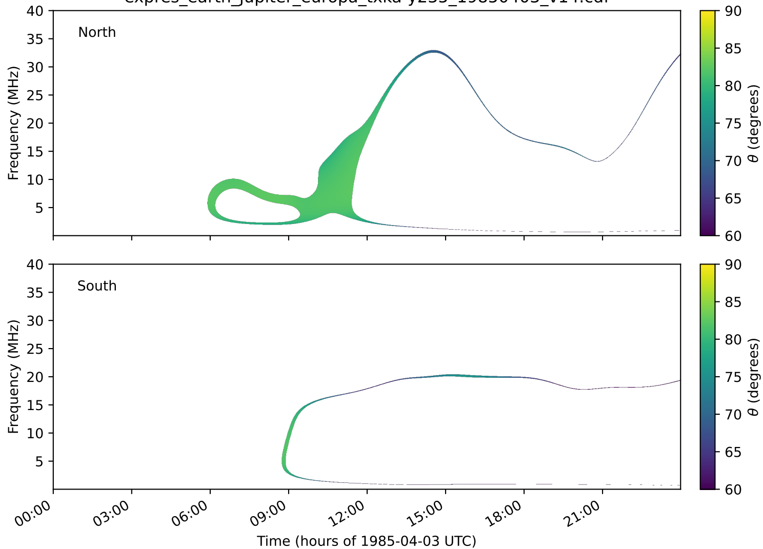
expres_earth_jupiter_europa_txka-y235_19850403_v14.cdf
