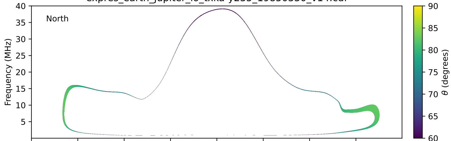
expres_earth_jupiter_io_txka-y235_19850330_v14.cdf
