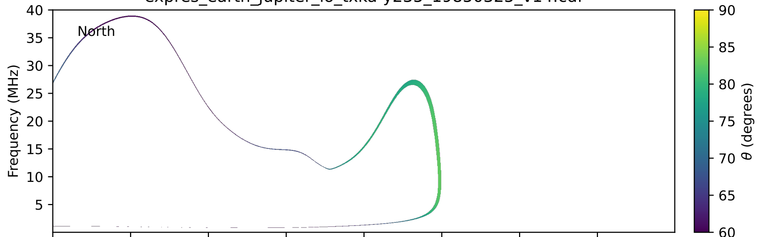
expres_earth_jupiter_io_txka-y235_19850325_v14.cdf
