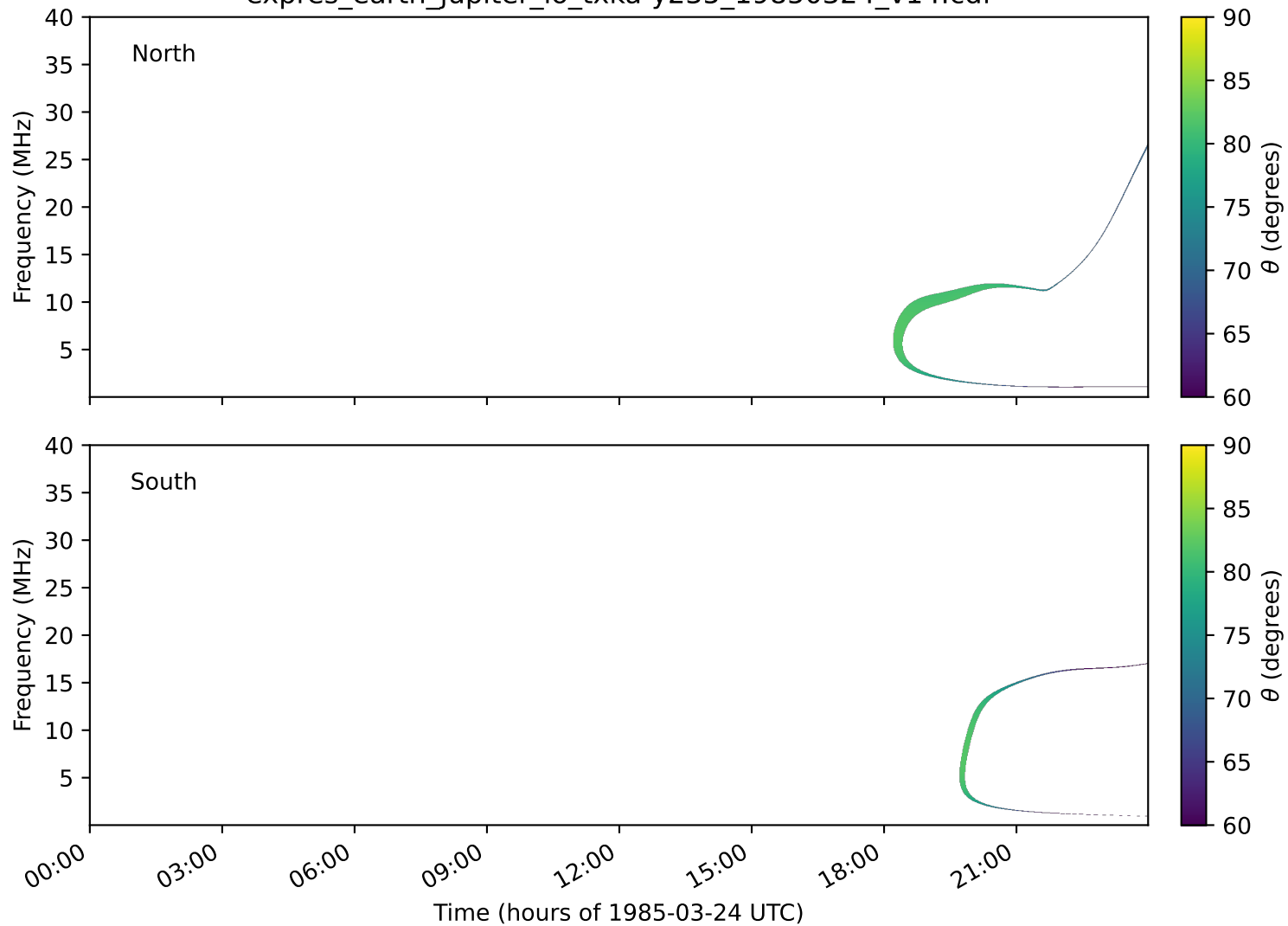
expres_earth_jupiter_io_txka-y235_19850324_v14.cdf
