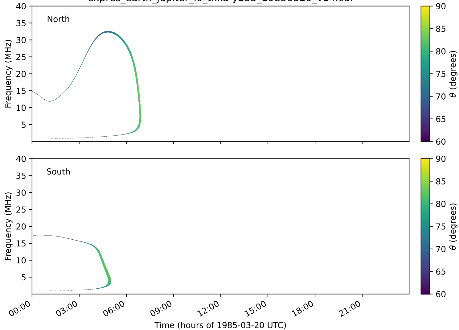
expres_earth_jupiter_io_txka-y235_19850320_v14.cdf
