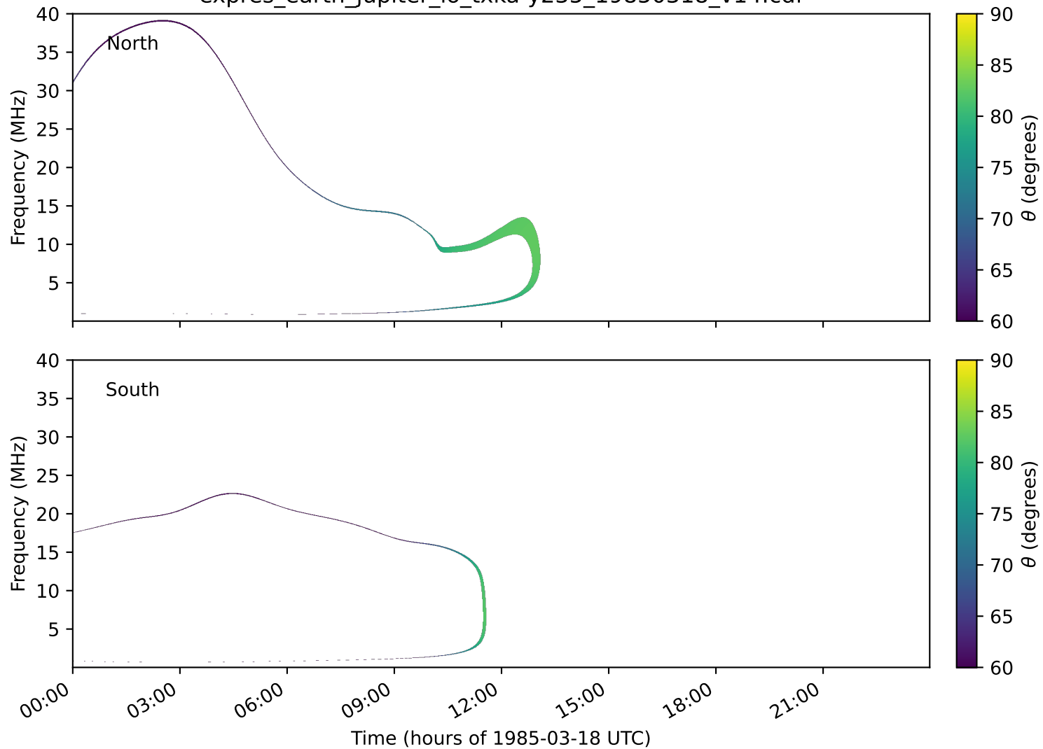
expres_earth_jupiter_io_txka-y235_19850318_v14.cdf
