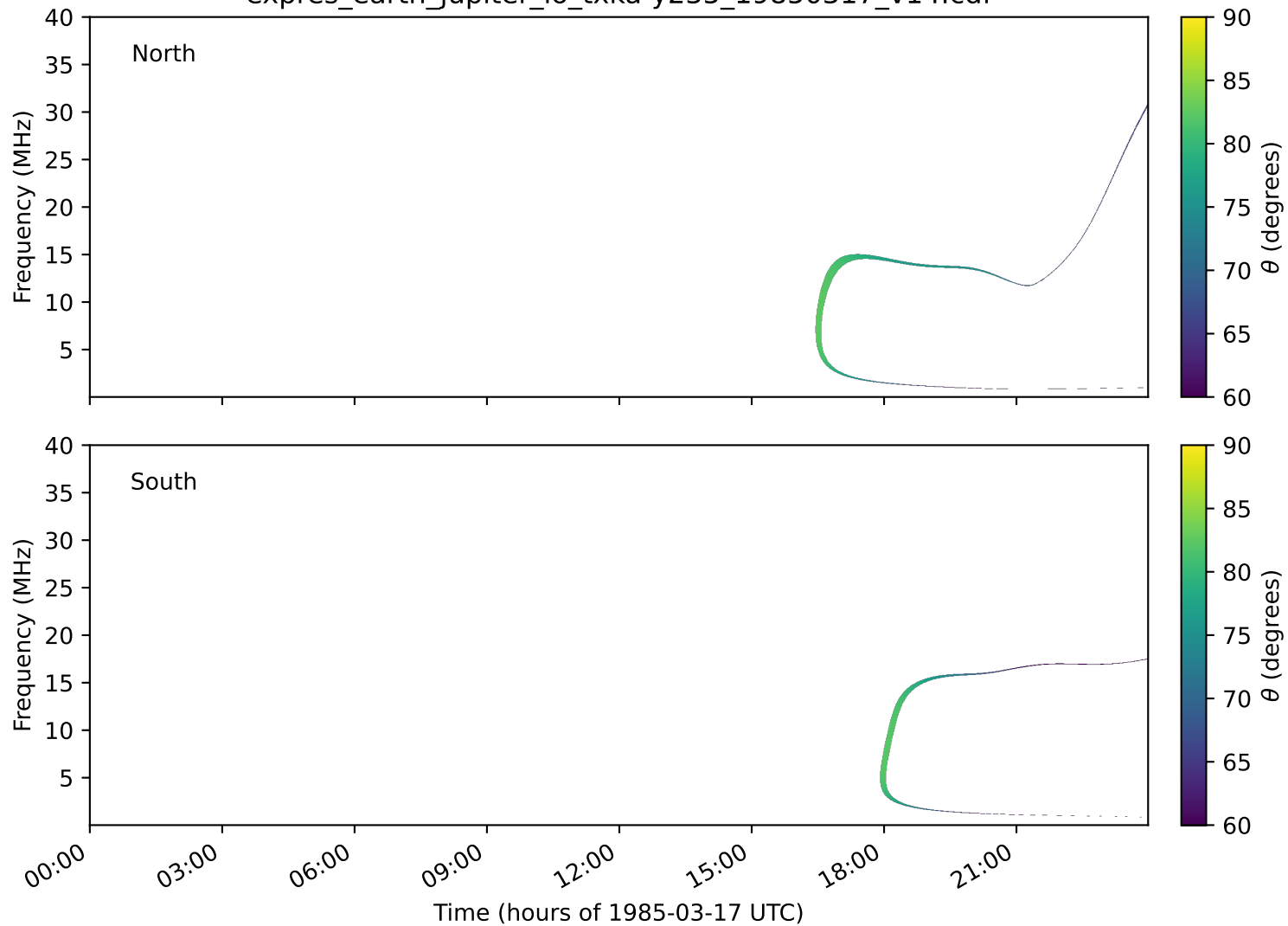
expres_earth_jupiter_io_txka-y235_19850317_v14.cdf
