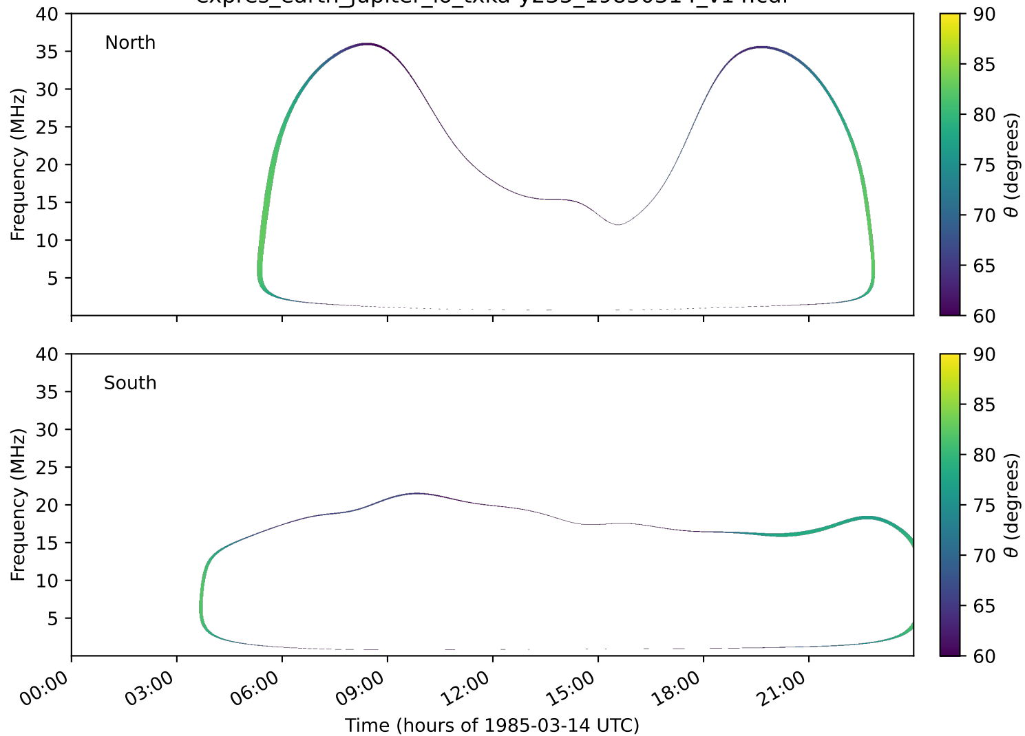
expres_earth_jupiter_io_txka-y235_19850314_v14.cdf
