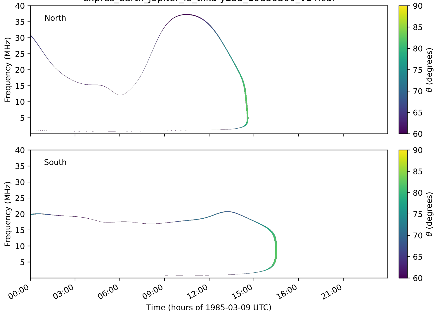
expres_earth_jupiter_io_txka-y235_19850309_v14.cdf
