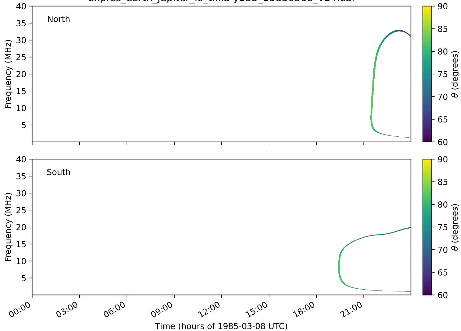
expres_earth_jupiter_io_txka-y235_19850308_v14.cdf
