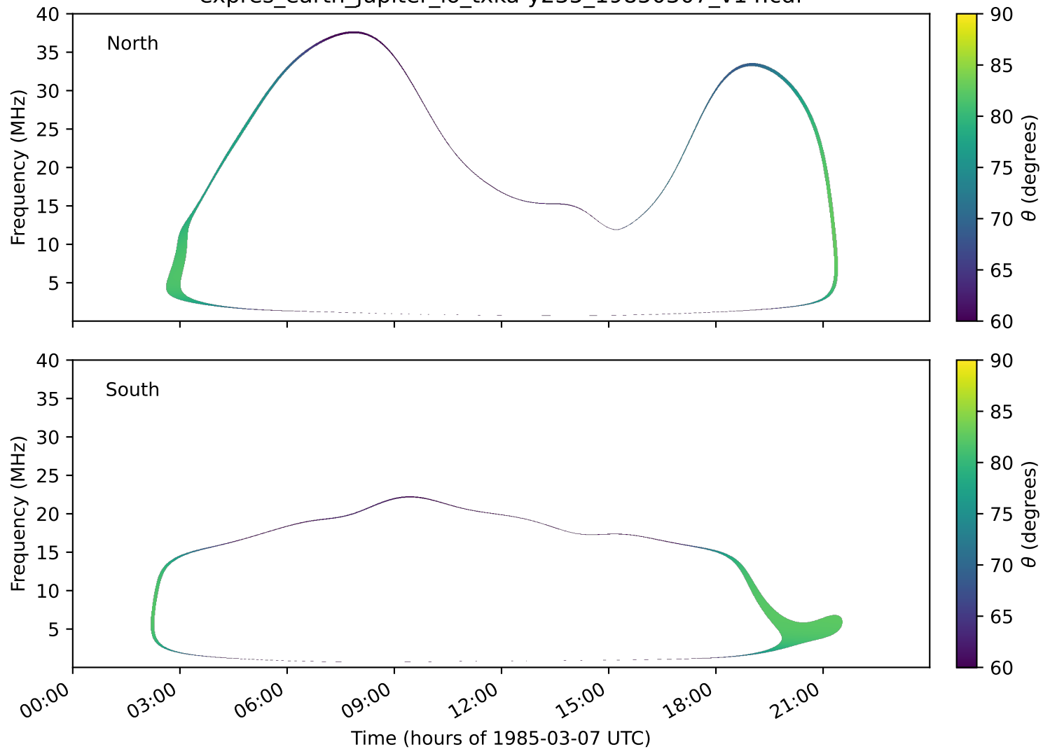
expres_earth_jupiter_io_txka-y235_19850307_v14.cdf
