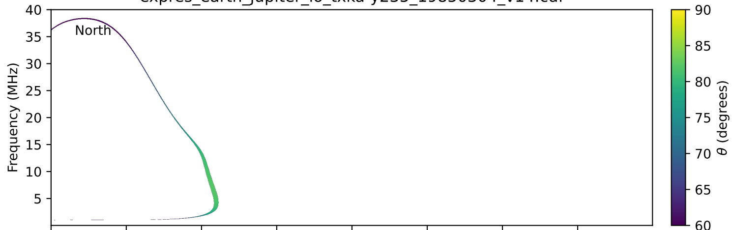
expres_earth_jupiter_io_txka-y235_19850304_v14.cdf
