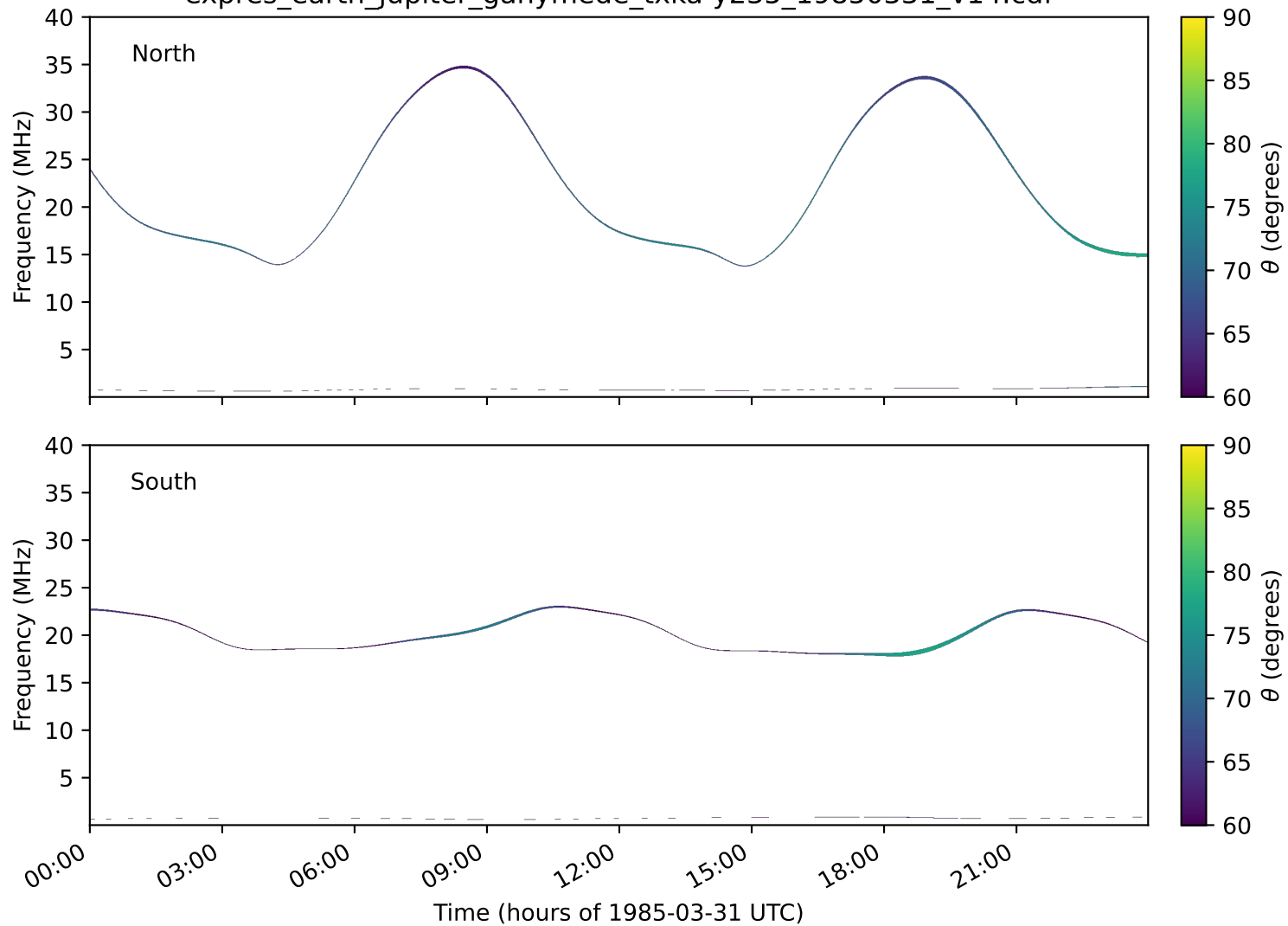
expres_earth_jupiter_ganymede_txka-y235_19850331_v14.cdf
