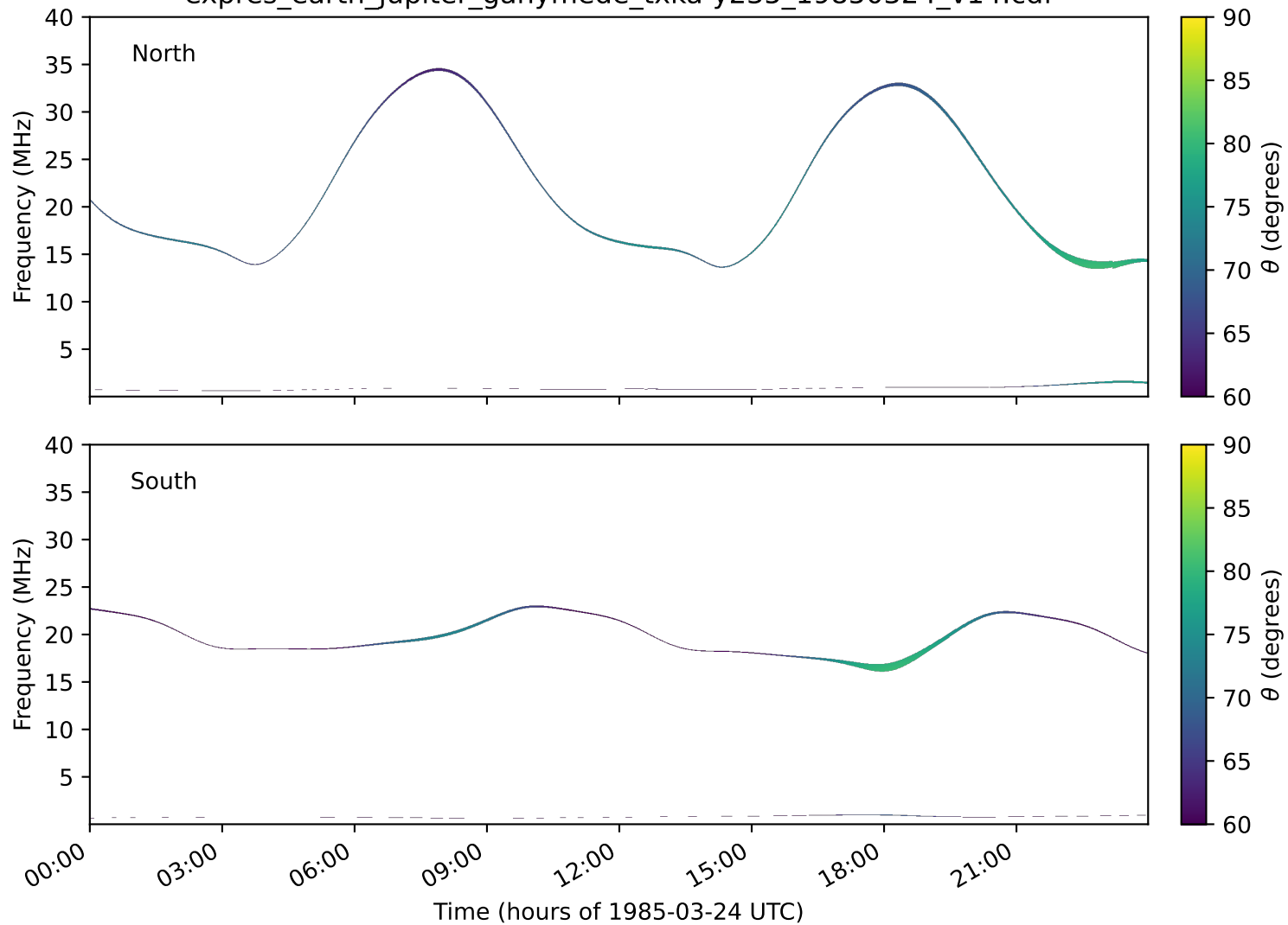
expres_earth_jupiter_ganymede_txka-y235_19850324_v14.cdf
