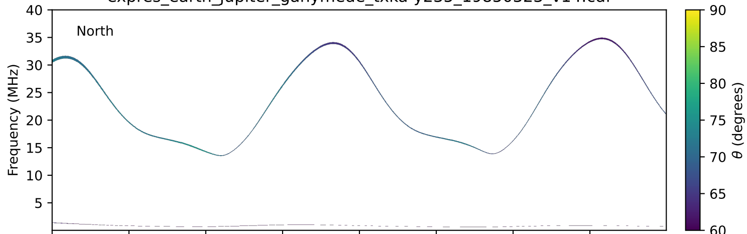
expres_earth_jupiter_ganymede_txka-y235_19850323_v14.cdf
