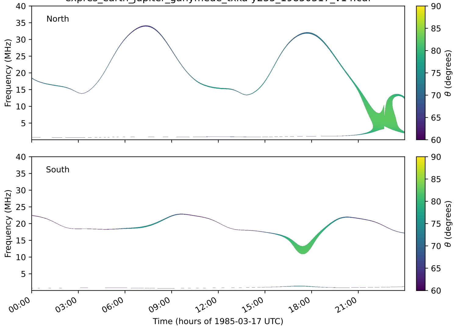
expres_earth_jupiter_ganymede_txka-y235_19850317_v14.cdf
