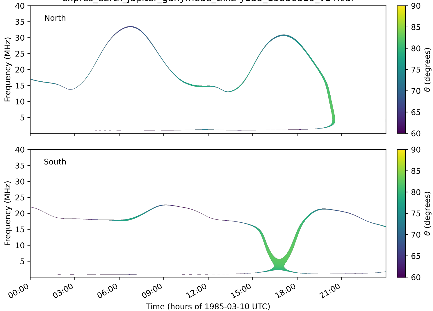
expres_earth_jupiter_ganymede_txka-y235_19850310_v14.cdf
