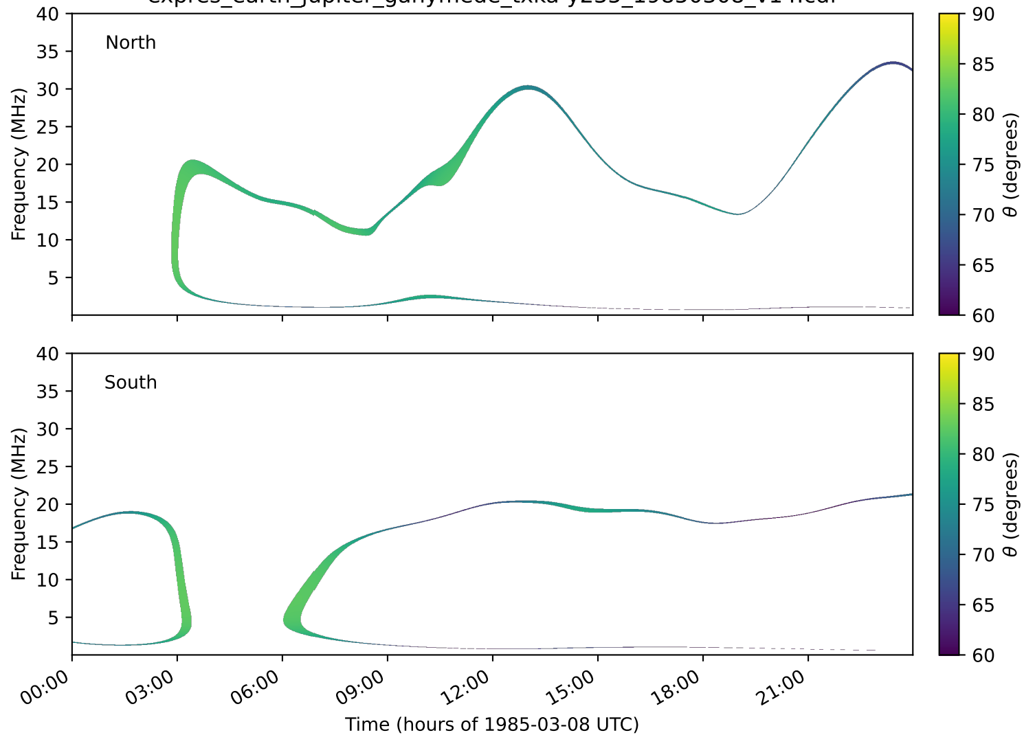
expres_earth_jupiter_ganymede_txka-y235_19850308_v14.cdf
