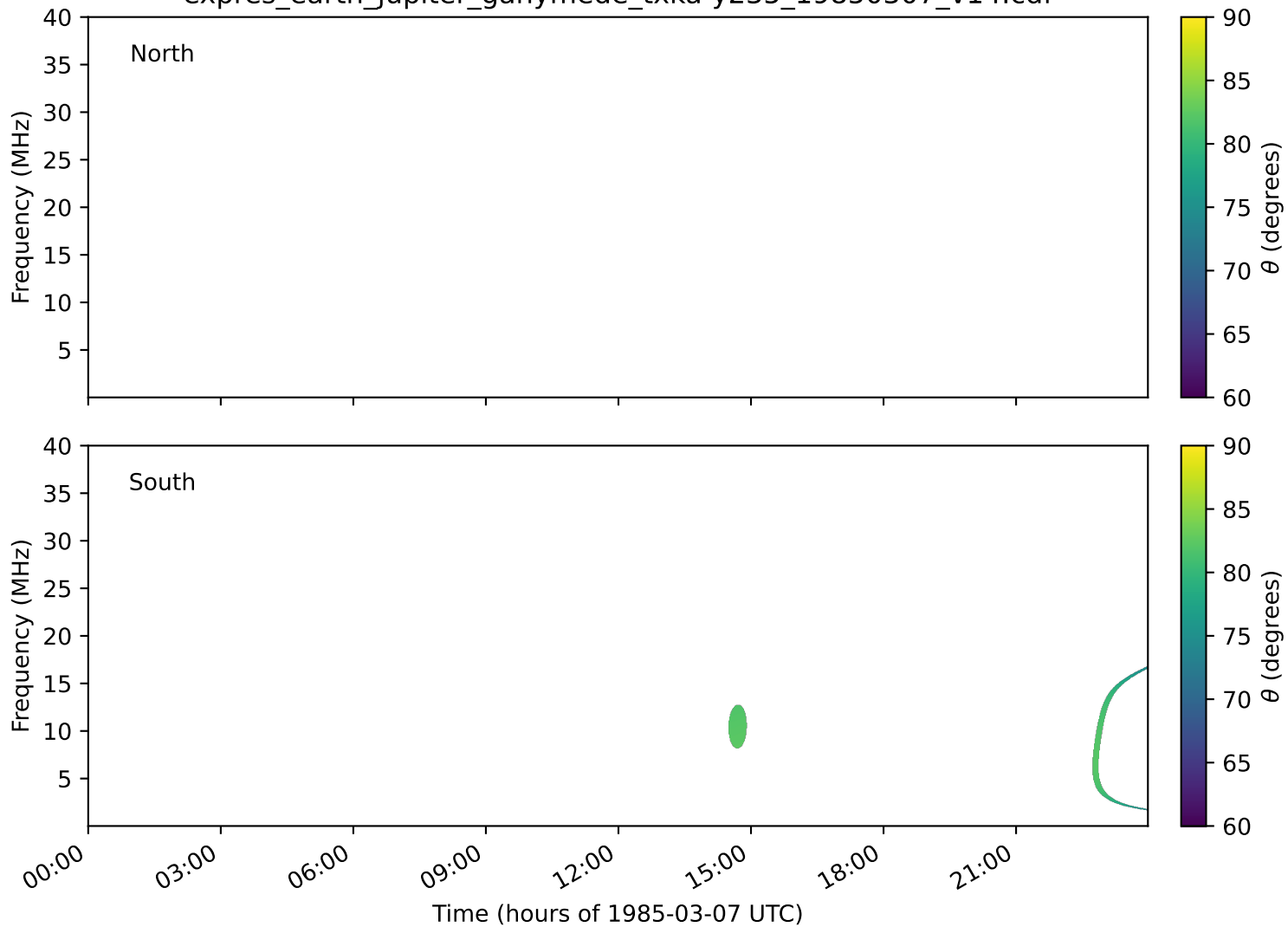
expres_earth_jupiter_ganymede_txka-y235_19850307_v14.cdf
