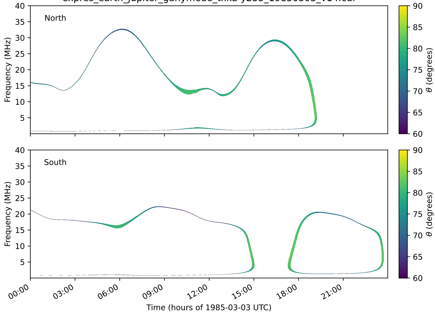
expres_earth_jupiter_ganymede_txka-y235_19850303_v14.cdf
