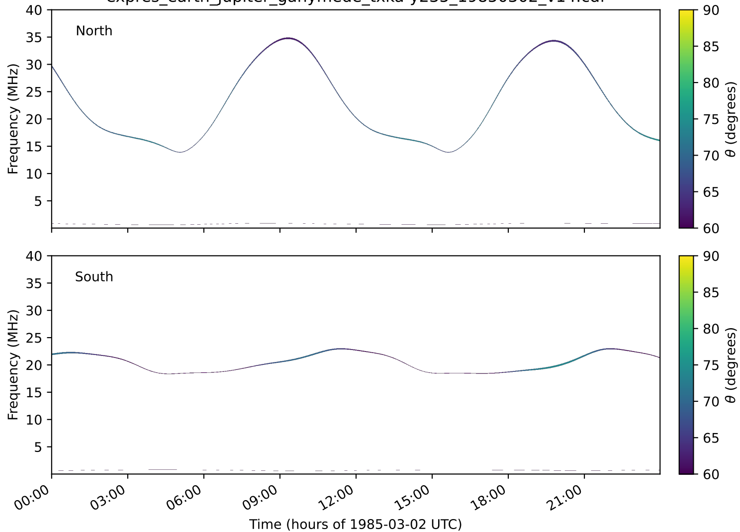
expres_earth_jupiter_ganymede_txka-y235_19850302_v14.cdf
