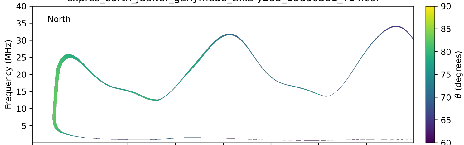
expres_earth_jupiter_ganymede_txka-y235_19850301_v14.cdf
