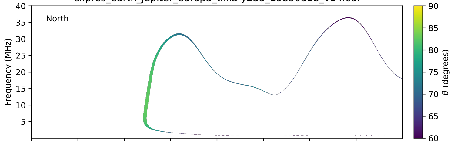
expres_earth_jupiter_europa_txka-y235_19850328_v14.cdf
