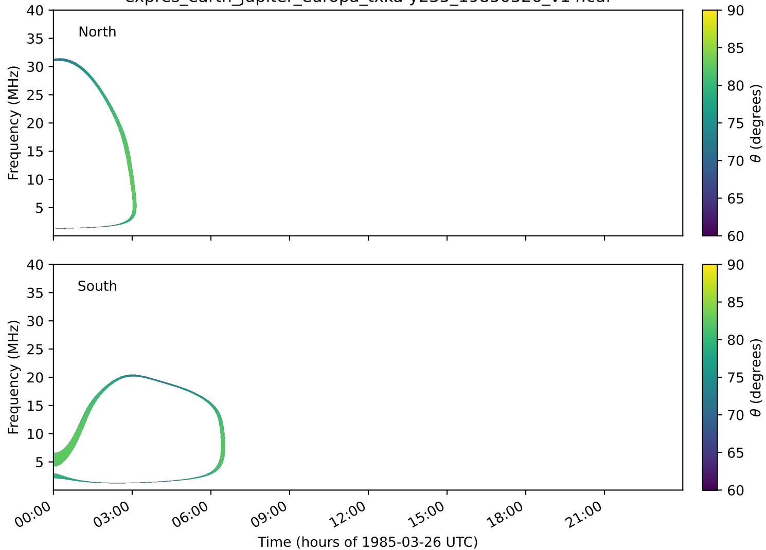
expres_earth_jupiter_europa_txka-y235_19850326_v14.cdf
