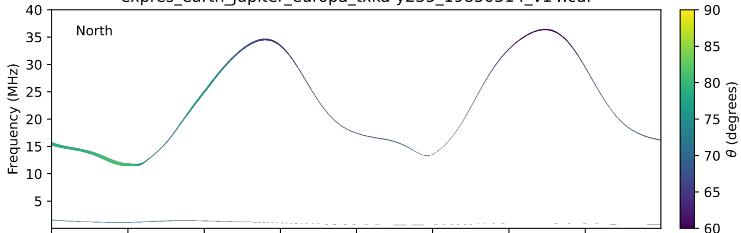
expres_earth_jupiter_europa_txka-y235_19850314_v14.cdf
