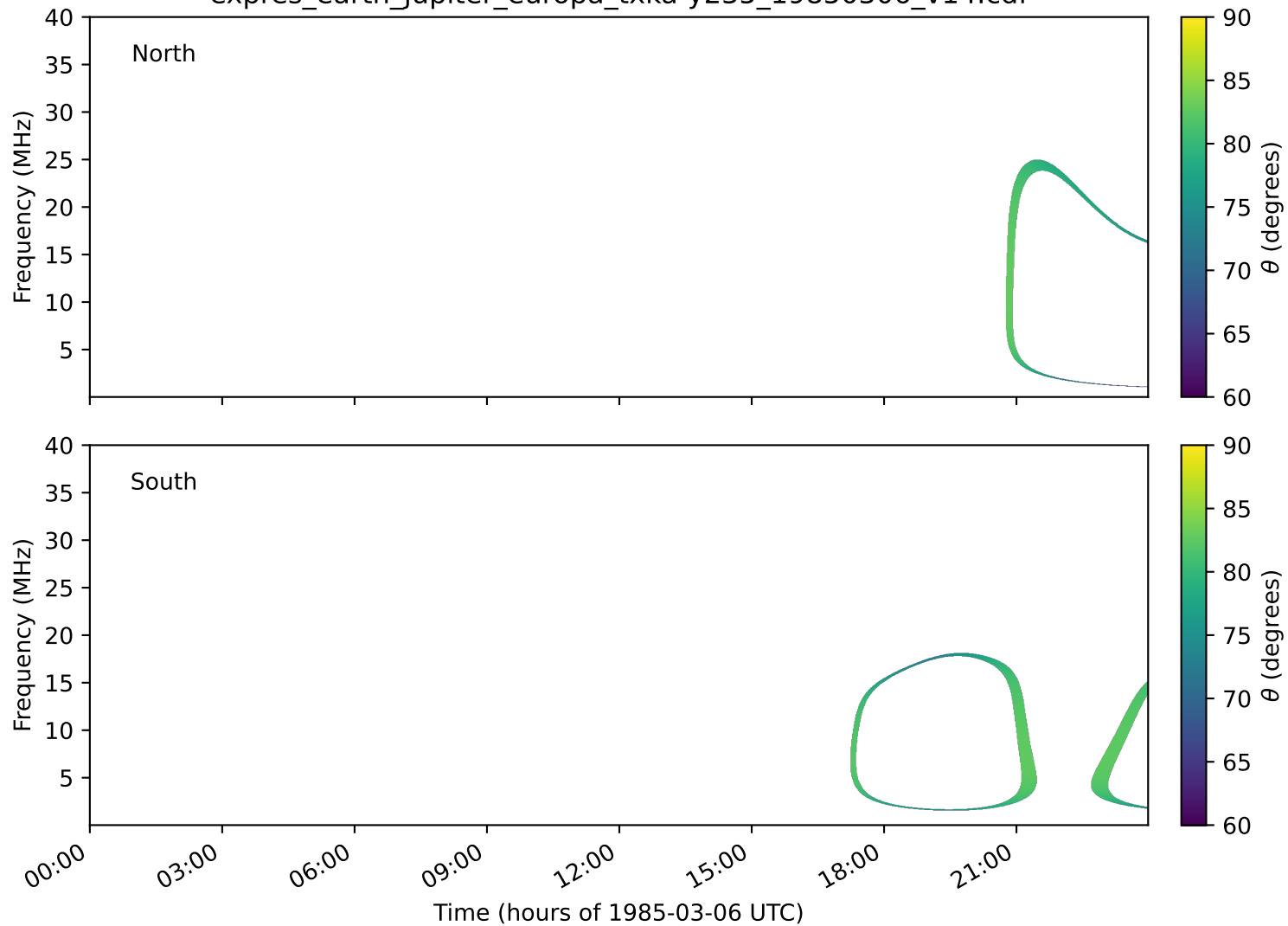
expres_earth_jupiter_europa_txka-y235_19850306_v14.cdf
