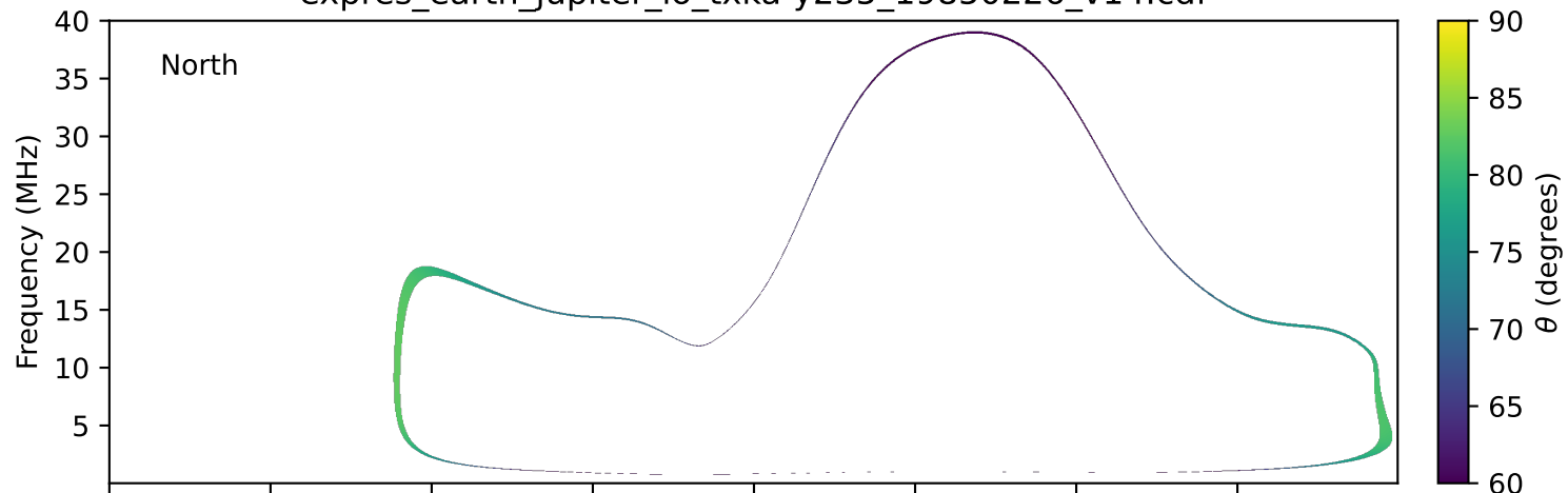
expres_earth_jupiter_io_txka-y235_19850226_v14.cdf
