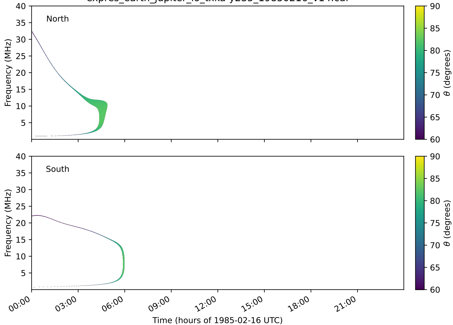
expres_earth_jupiter_io_txka-y235_19850216_v14.cdf
