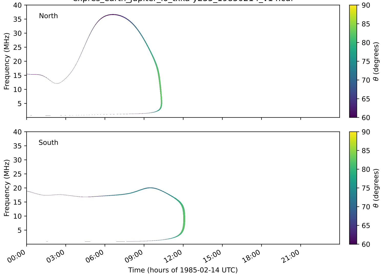
expres_earth_jupiter_io_txka-y235_19850214_v14.cdf
