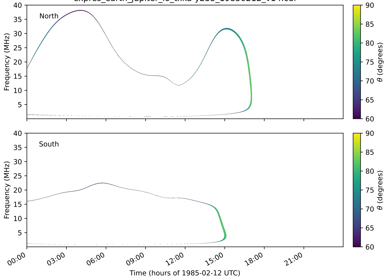
expres_earth_jupiter_io_txka-y235_19850212_v14.cdf
