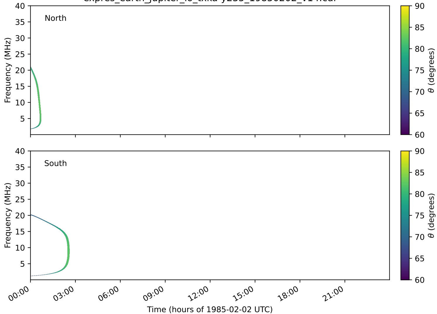
expres_earth_jupiter_io_txka-y235_19850202_v14.cdf
