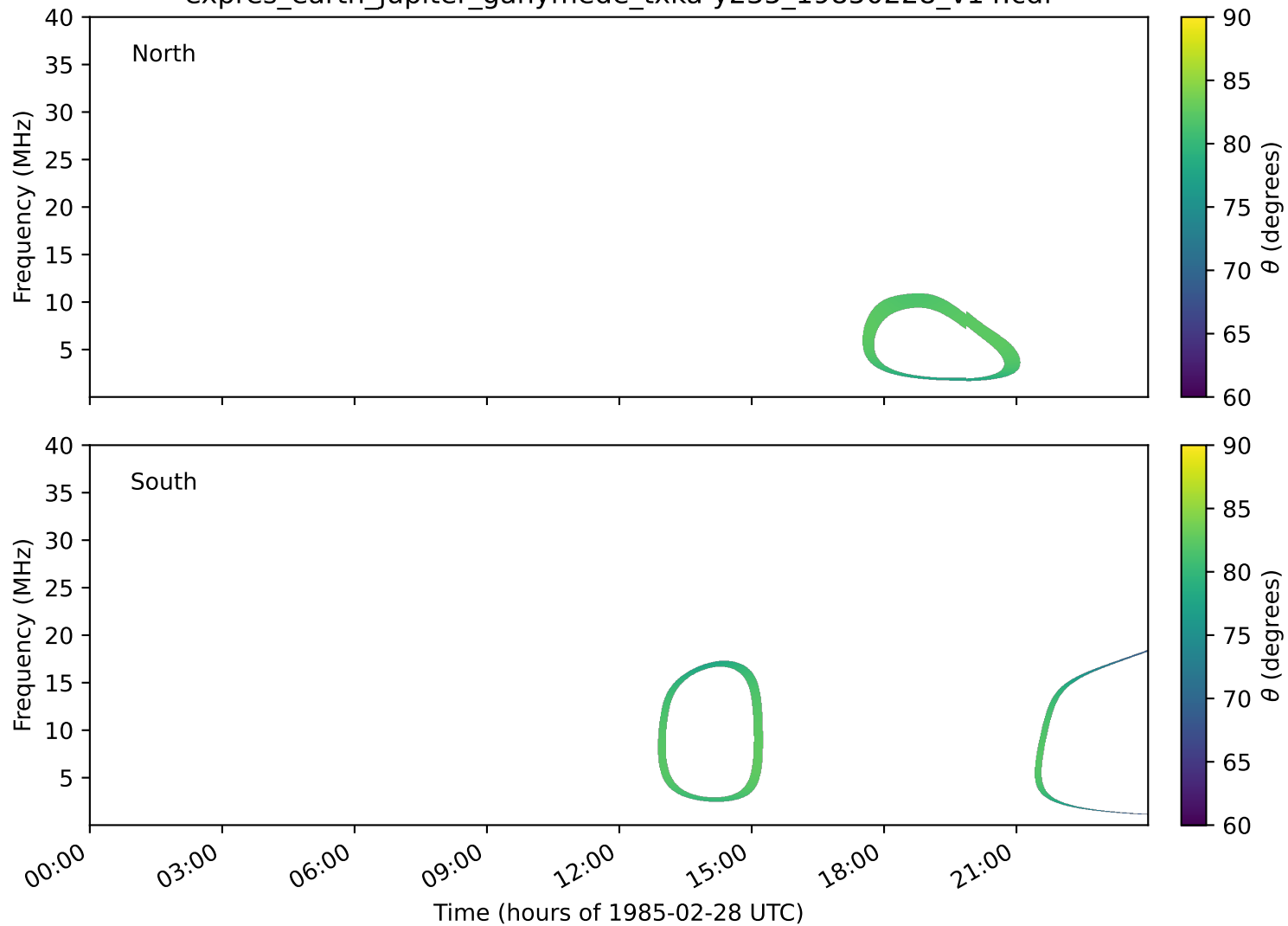
expres_earth_jupiter_ganymede_txka-y235_19850228_v14.cdf
