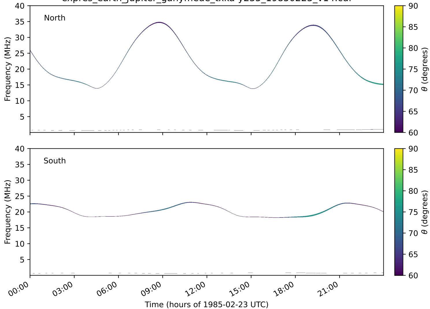
expres_earth_jupiter_ganymede_txka-y235_19850223_v14.cdf
