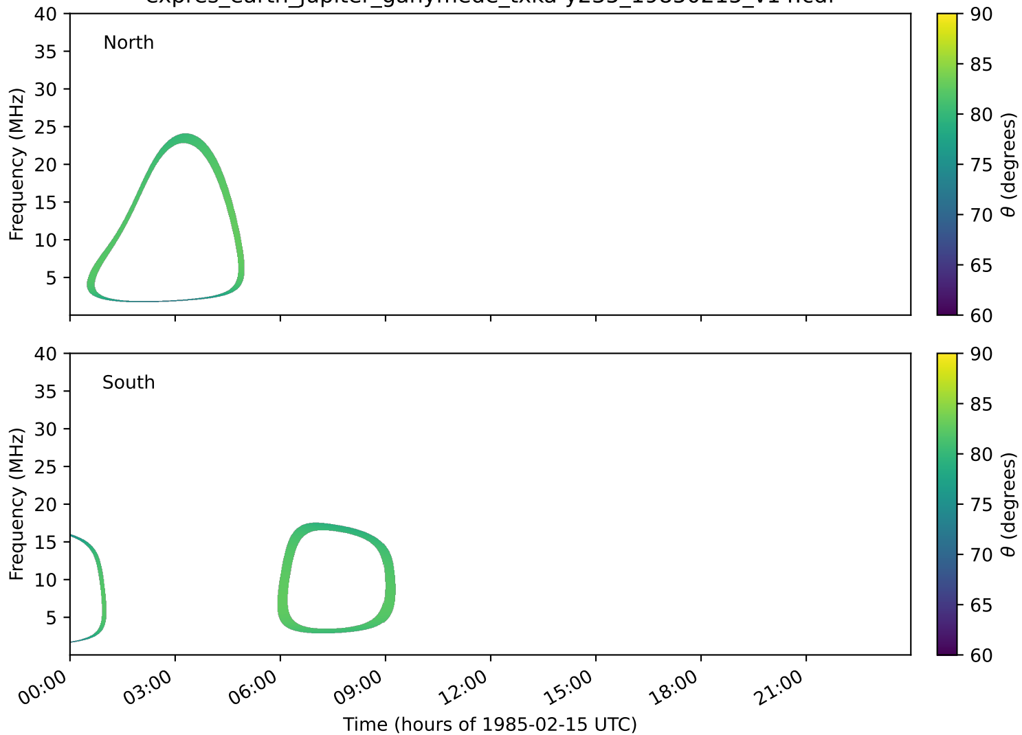
expres_earth_jupiter_ganymede_txka-y235_19850215_v14.cdf
