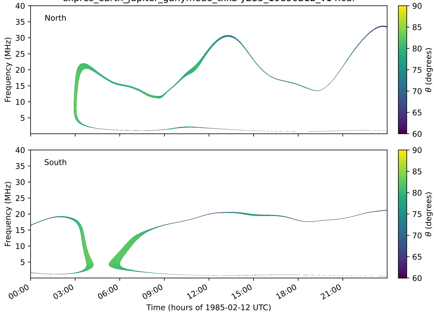
expres_earth_jupiter_ganymede_txka-y235_19850212_v14.cdf
