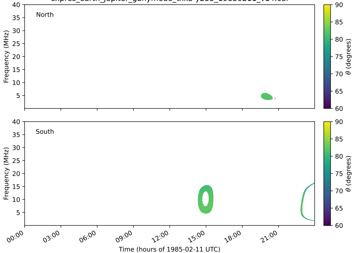
expres_earth_jupiter_ganymede_txka-y235_19850211_v14.cdf
