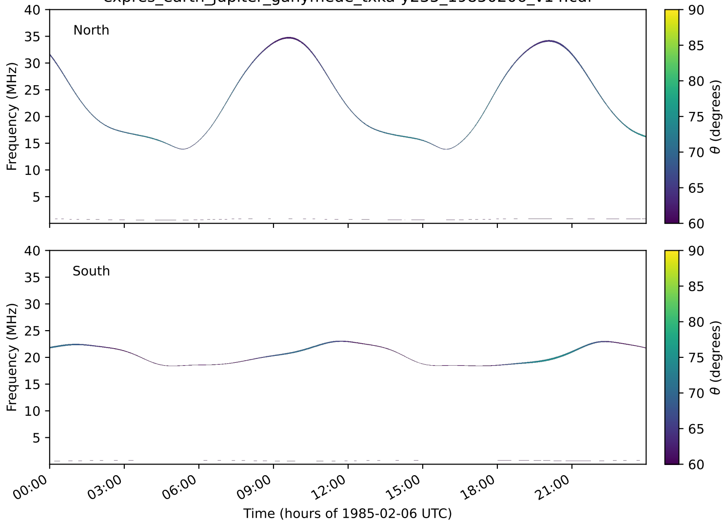
expres_earth_jupiter_ganymede_txka-y235_19850206_v14.cdf
