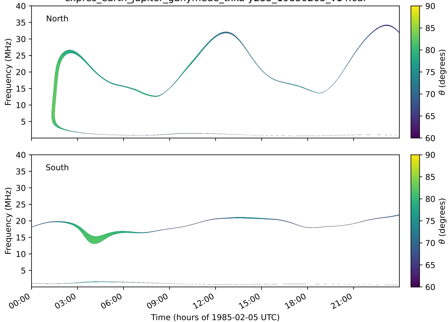
expres_earth_jupiter_ganymede_txka-y235_19850205_v14.cdf
