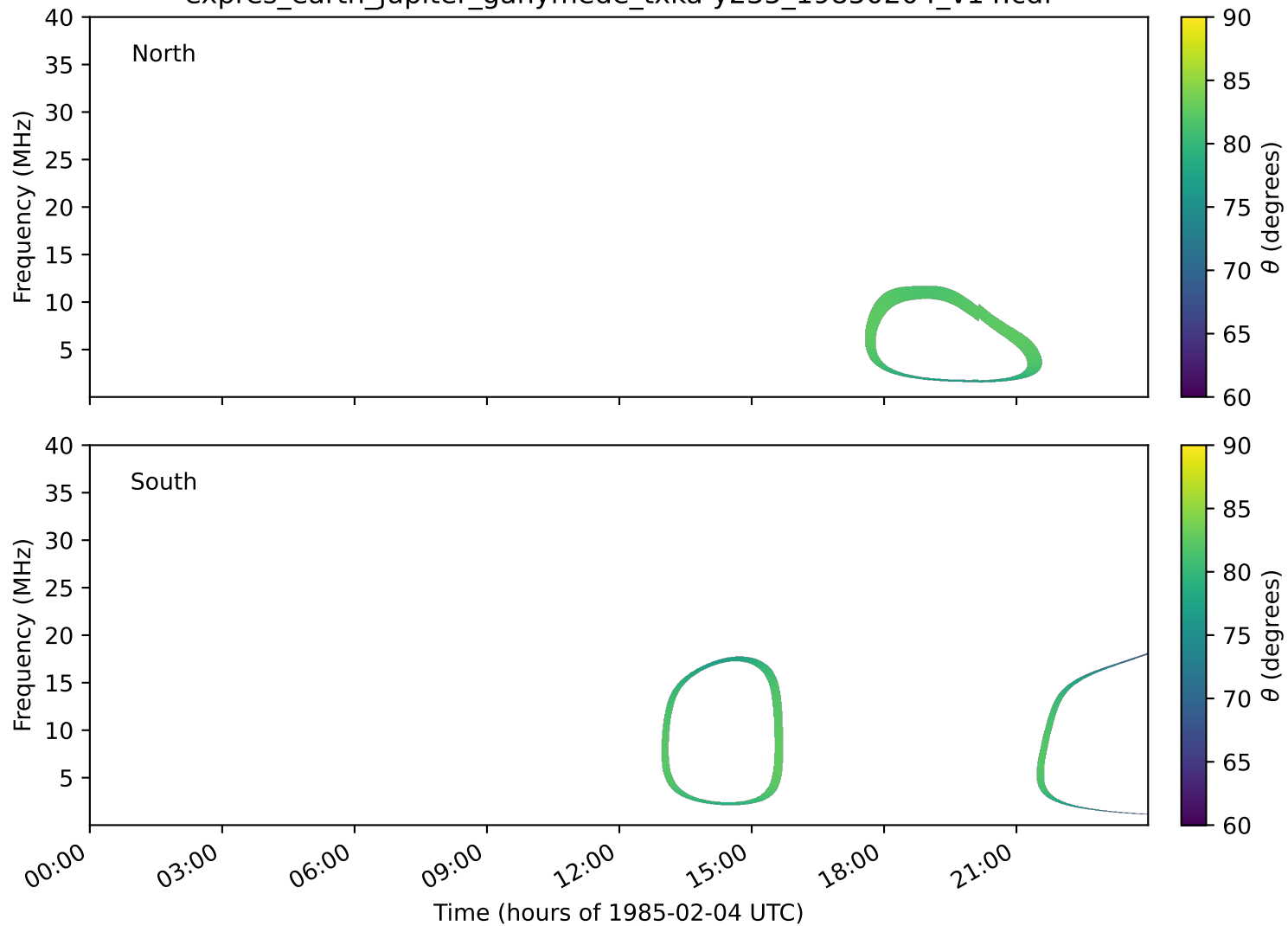
expres_earth_jupiter_ganymede_txka-y235_19850204_v14.cdf
